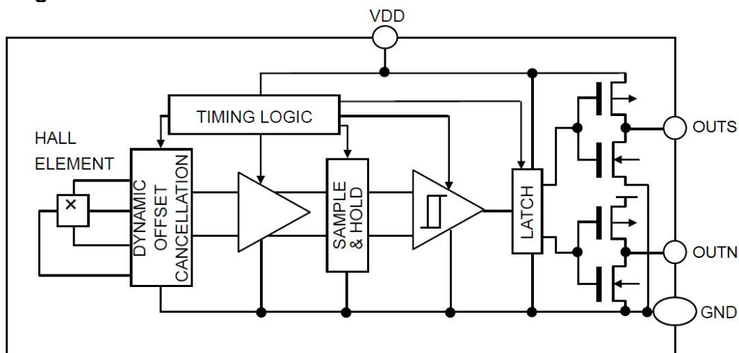
Figure 2, Block Diagram of AS1828A
